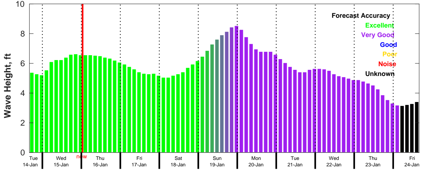
CMEMS Wave Forecast for NDBC 46011 from 14-Jan-2025 16:00:00 to 24-Jan-2025 16:00:00
