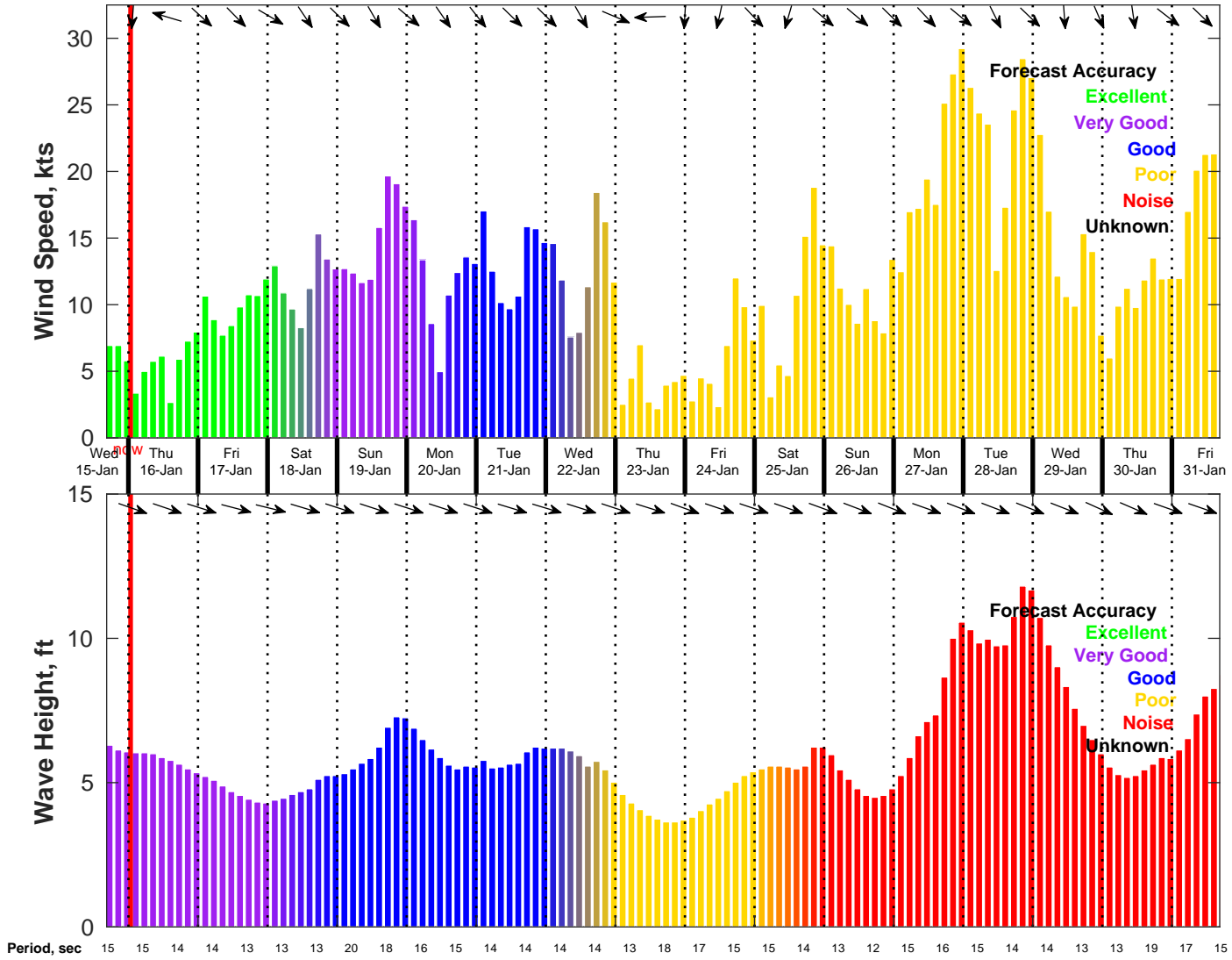
Wind & Wave Forecast for NDBC 46011 from 15-Jan-2025 16:00:00 to 31-Jan-2025 16:00:00
