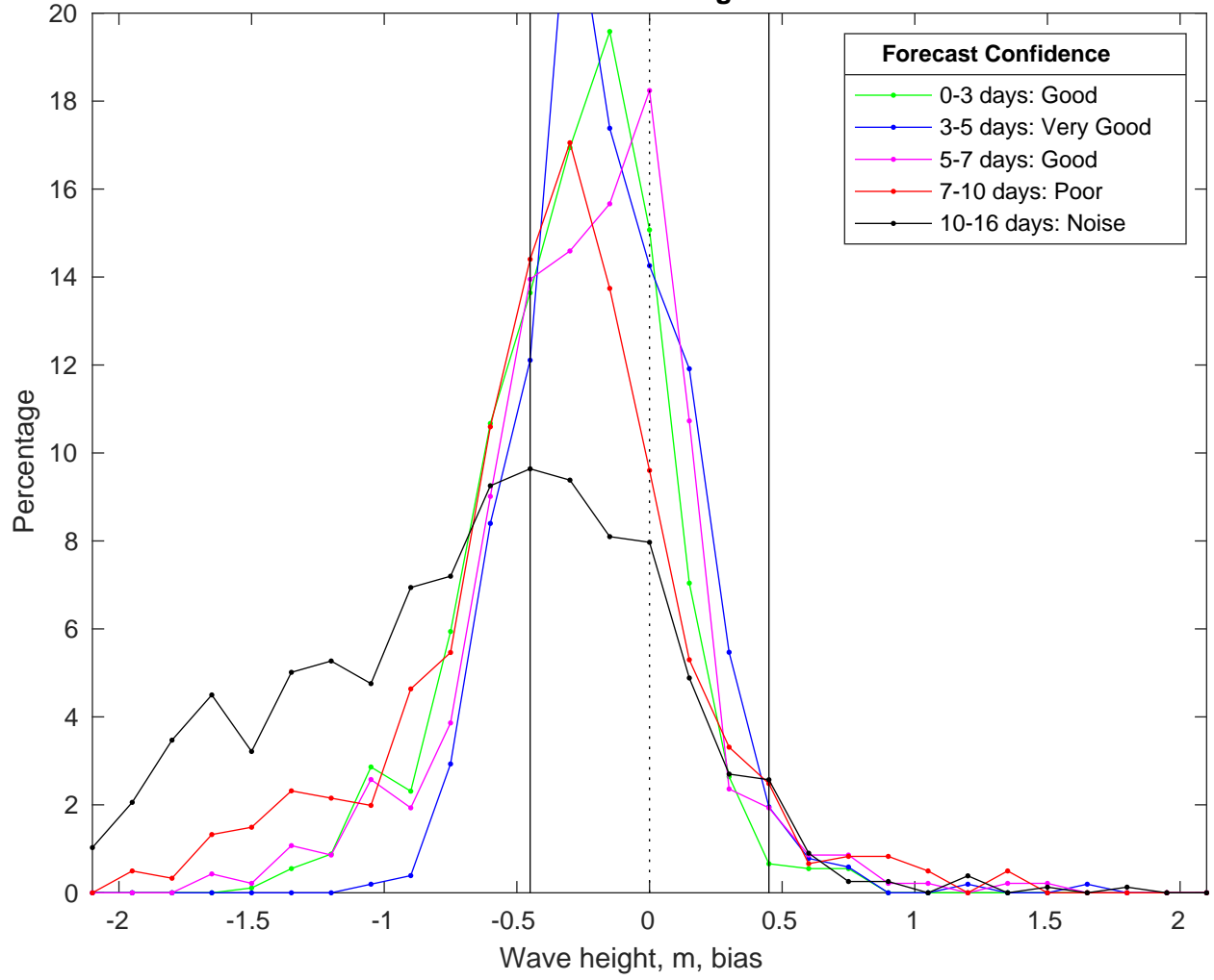
NDBC 46028 vs GFSWaves Bias Histogram: 16-Jan-2025
