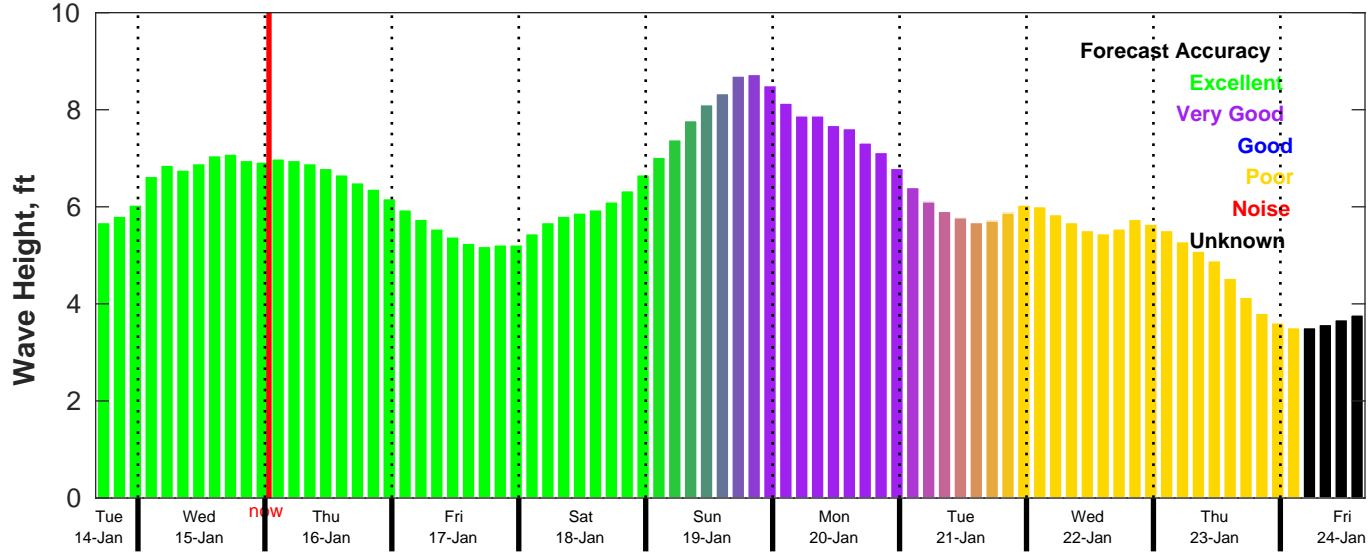
CMEMS Wave Forecast for NDBC 46028 from 14-Jan-2025 16:00:00 to 24-Jan-2025 16:00:00
