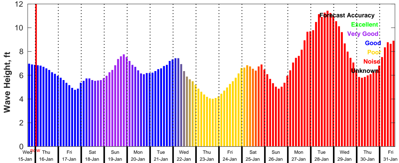
GFS Wave Forecast for NDBC 46028 from 15-Jan-2025 16:00:00 to 31-Jan-2025 16:00:00
