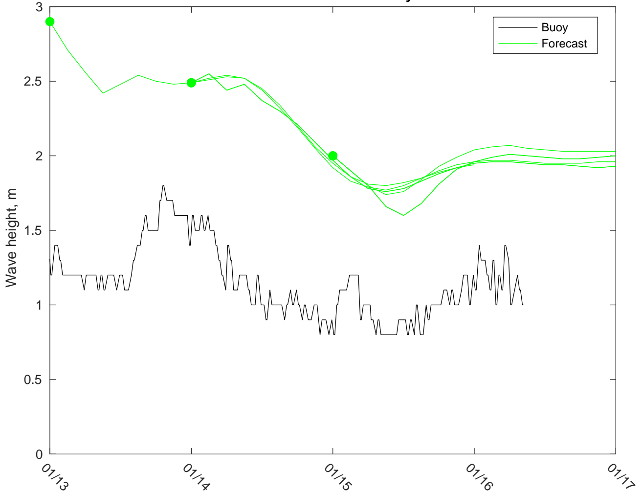
NDBC 46053 vs CMEMSWaves: 0 to 3 day forecast
