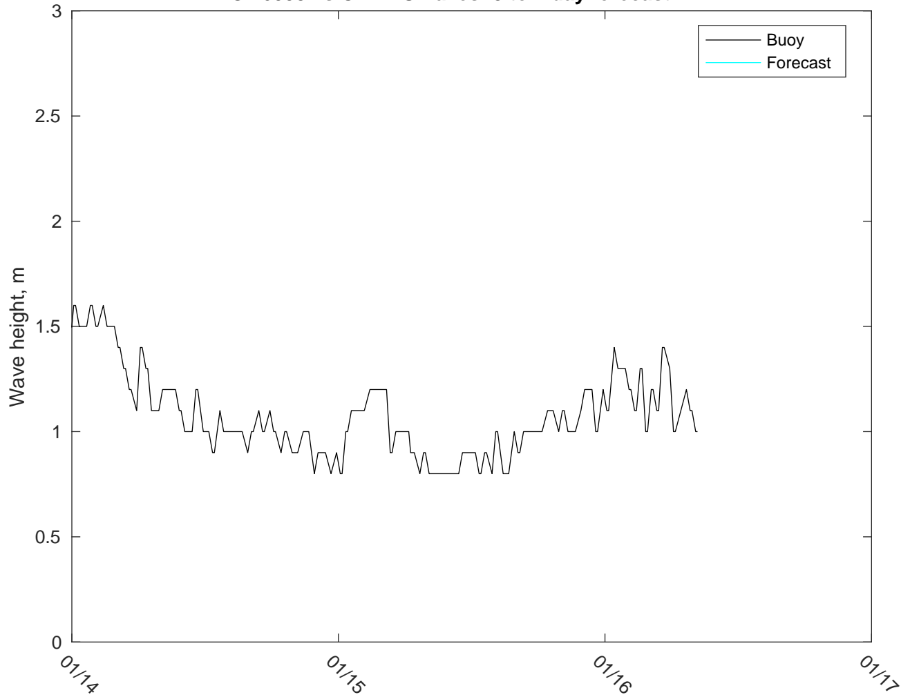
NDBC 46053 vs CMEMSWaves: 5 to 7 day forecast
