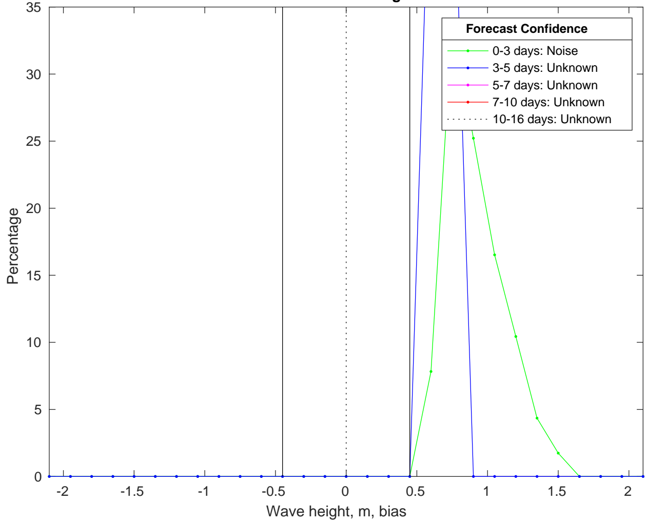
NDBC 46053 vs CMEMSWaves Bias Histogram: 16-Jan-2025
