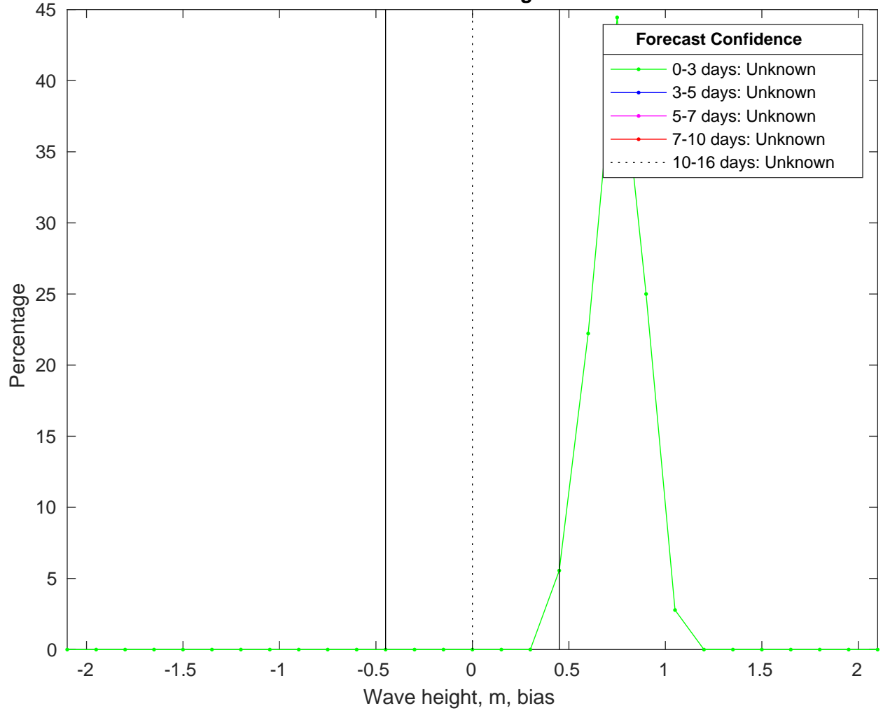
NDBC 46053 vs GFSWaves Bias Histogram: 16-Jan-2025
