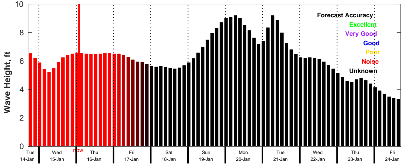
CMEMS Wave Forecast for NDBC 46053 from 14-Jan-2025 17:00:00 to 24-Jan-2025 17:00:00
