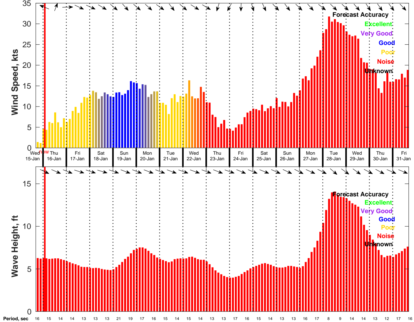
Wind & Wave Forecast for NDBC 46053 from 15-Jan-2025 17:00:00 to 31-Jan-2025 17:00:00
