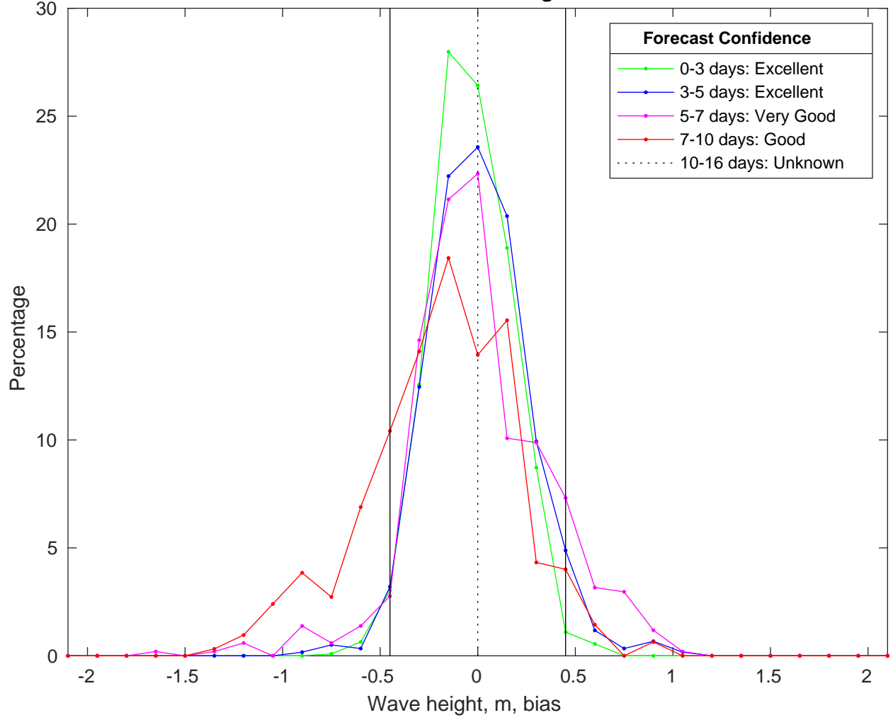
NDBC 46054 vs CMEMSWaves Bias Histogram: 16-Jan-2025
