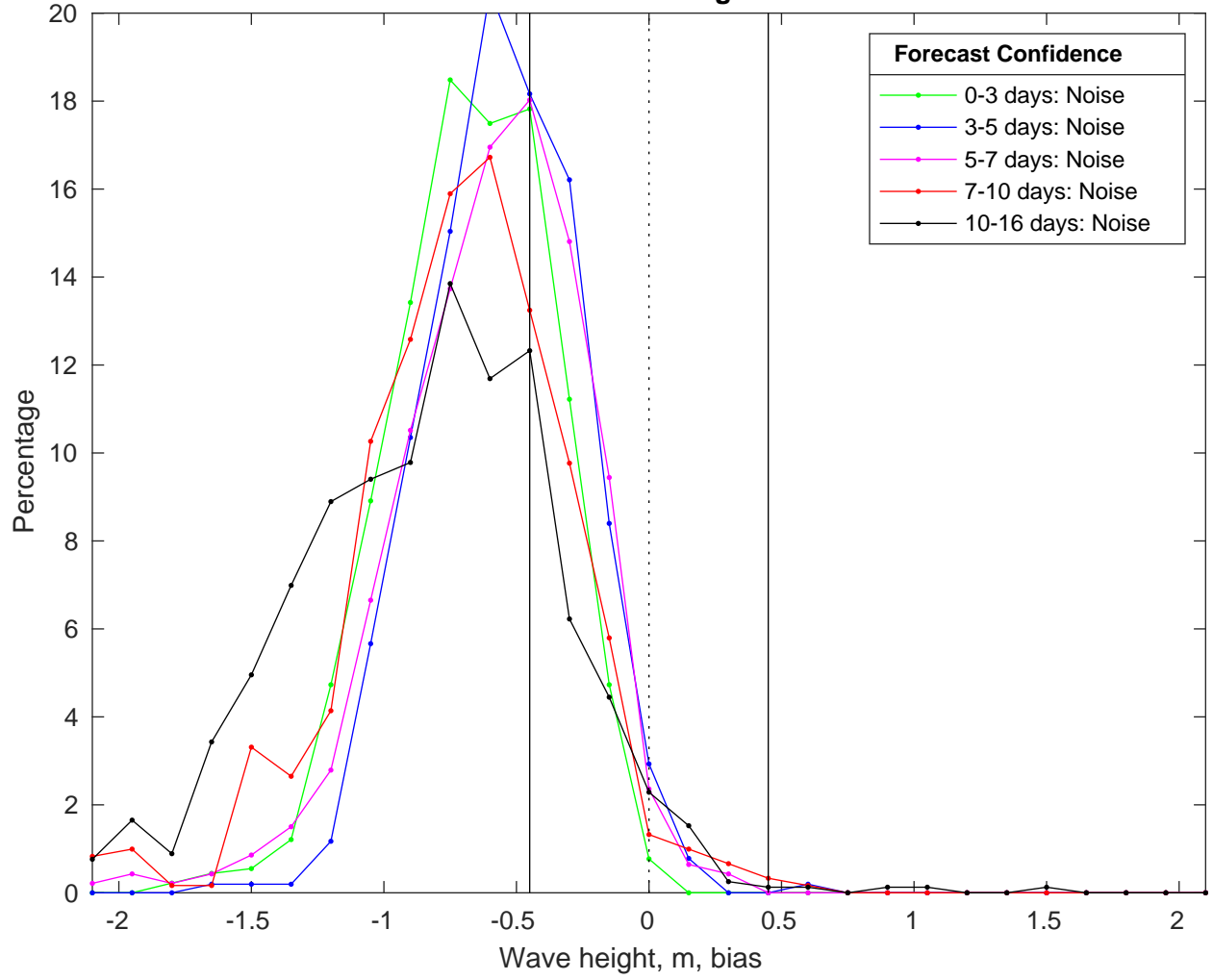
NDBC 46054 vs GFSWaves Bias Histogram: 16-Jan-2025
