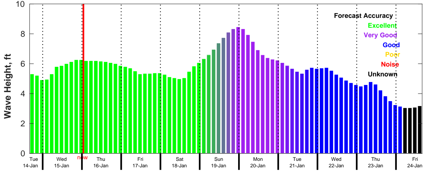
CMEMS Wave Forecast for NDBC 46054 from 14-Jan-2025 16:00:00 to 24-Jan-2025 16:00:00
