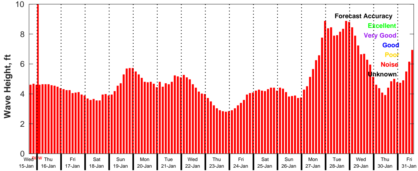
GFS Wave Forecast for NDBC 46054 from 15-Jan-2025 16:00:00 to 31-Jan-2025 16:00:00
