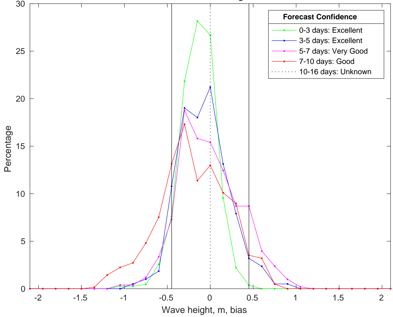
NDBC 46069 vs CMEMSWaves Bias Histogram: 16-Jan-2025
