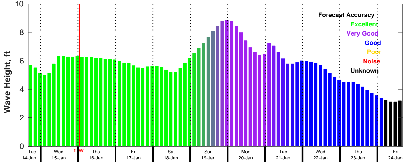
CMEMS Wave Forecast for NDBC 46069 from 14-Jan-2025 16:00:00 to 24-Jan-2025 16:00:00
