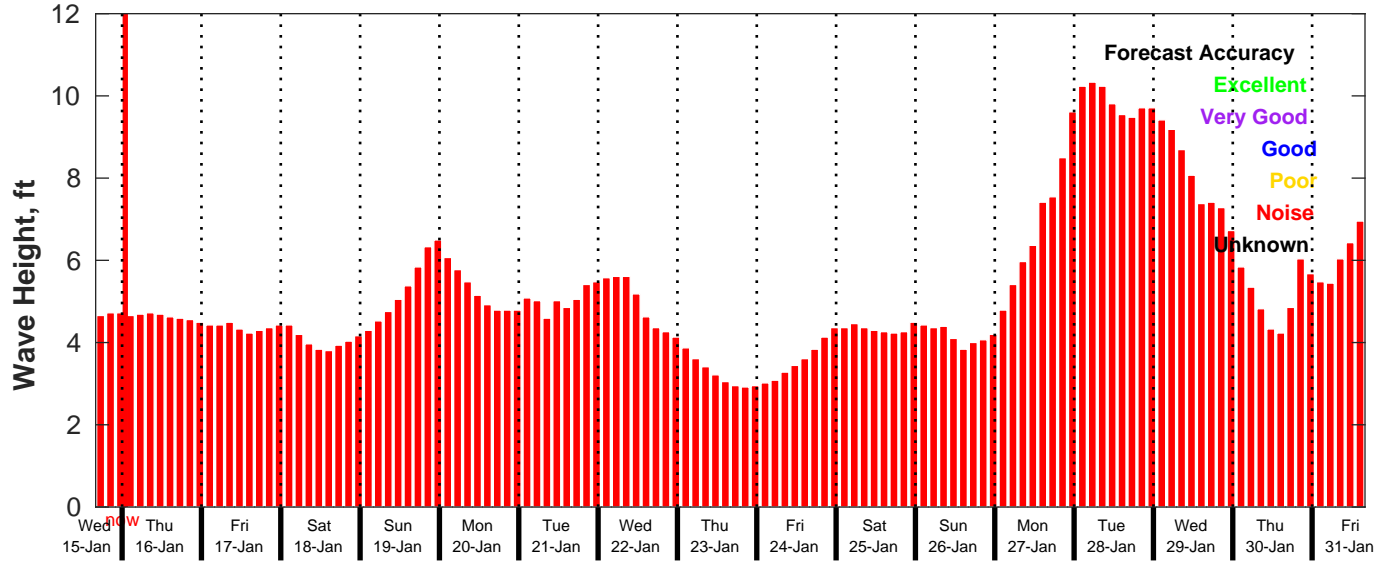
GFS Wave Forecast for NDBC 46069 from 15-Jan-2025 16:00:00 to 31-Jan-2025 16:00:00
