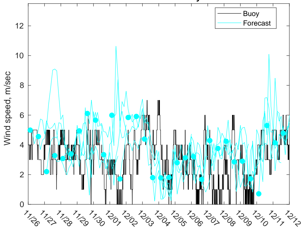
NDBC 46086 vs GFSWinds: 5 to 7 day forecast
