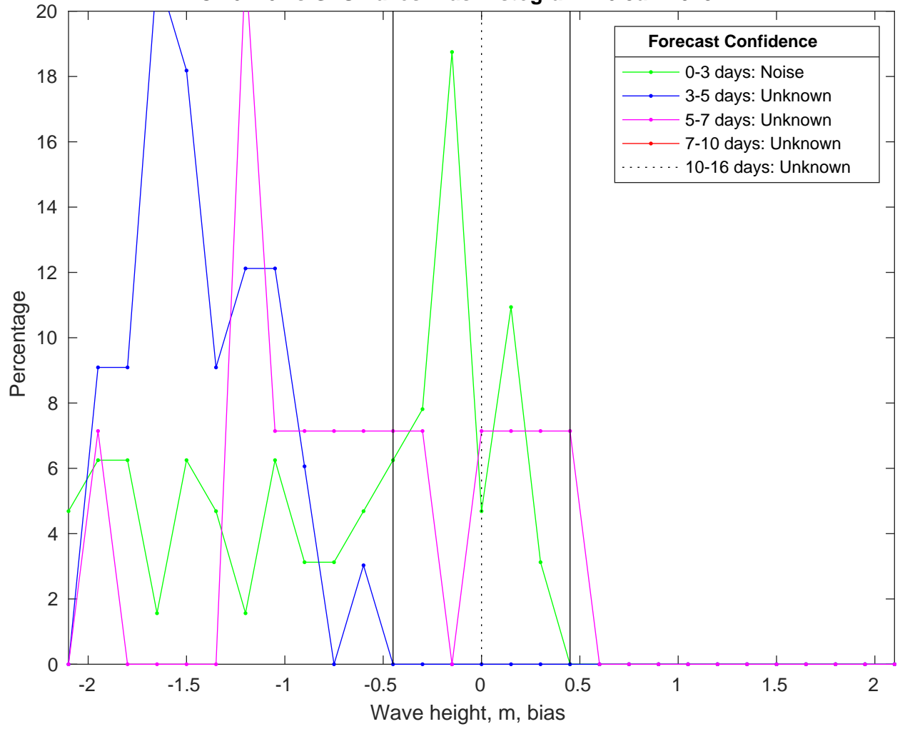
NDBC 46246 vs GFSWaves Bias Histogram: 16-Jan-2025
