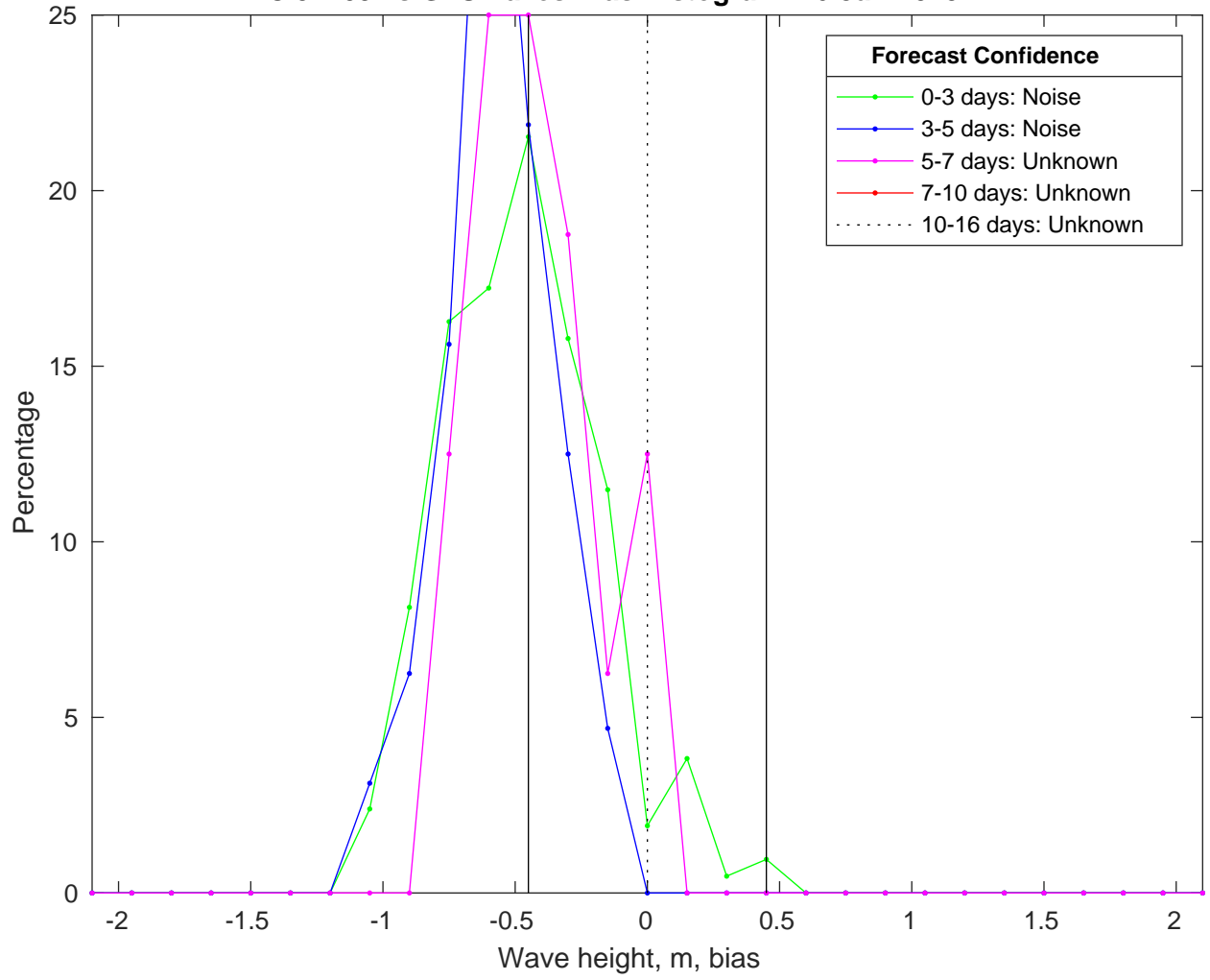
NDBC 51209 vs GFSWaves Bias Histogram: 16-Jan-2025
