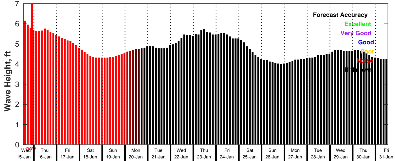
GFS Wave Forecast for NDBC 51209 from 15-Jan-2025 13:00:00 to 31-Jan-2025 13:00:00
