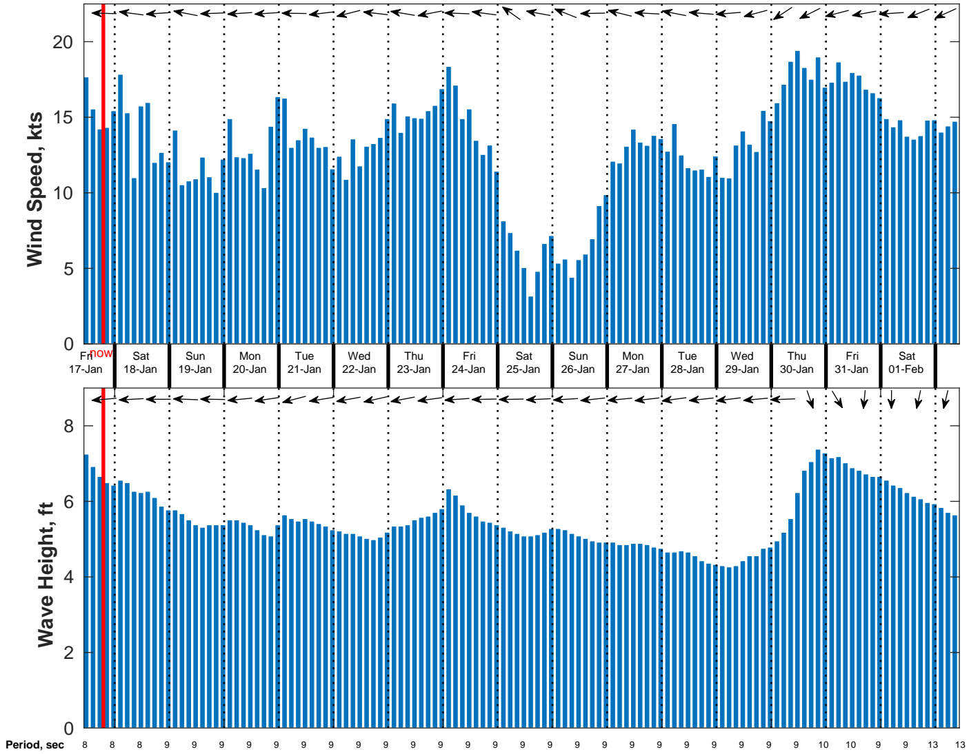
Wind & Wave Forecast for NDBC 52211 from 16-Jan-2025 10:00:00 to 01-Feb-2025 10:00:00
