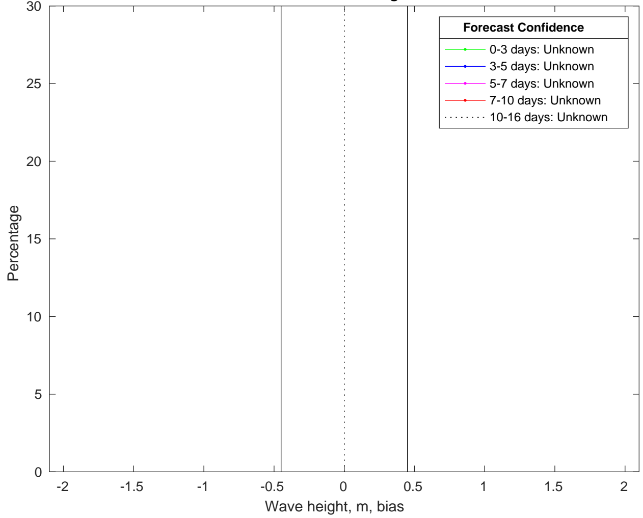
NDBC 52212 vs CMEMSWaves Bias Histogram: 16-Jan-2025
