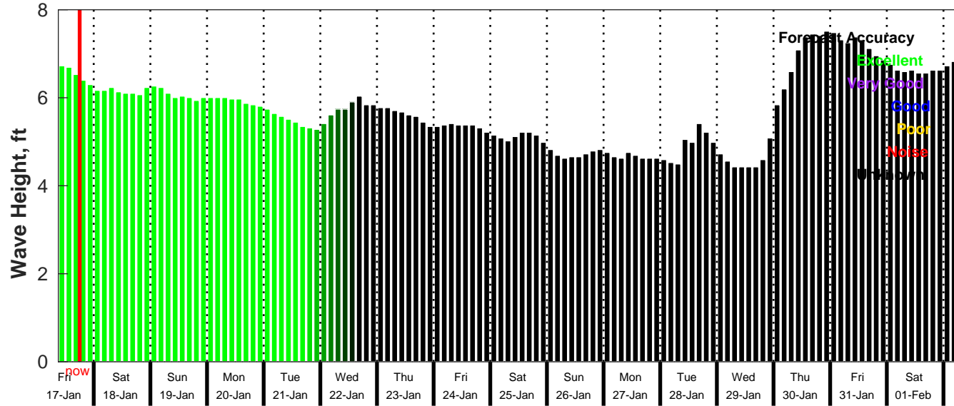
GFS Wave Forecast for NDBC 52212 from 16-Jan-2025 09:00:00 to 01-Feb-2025 09:00:00
