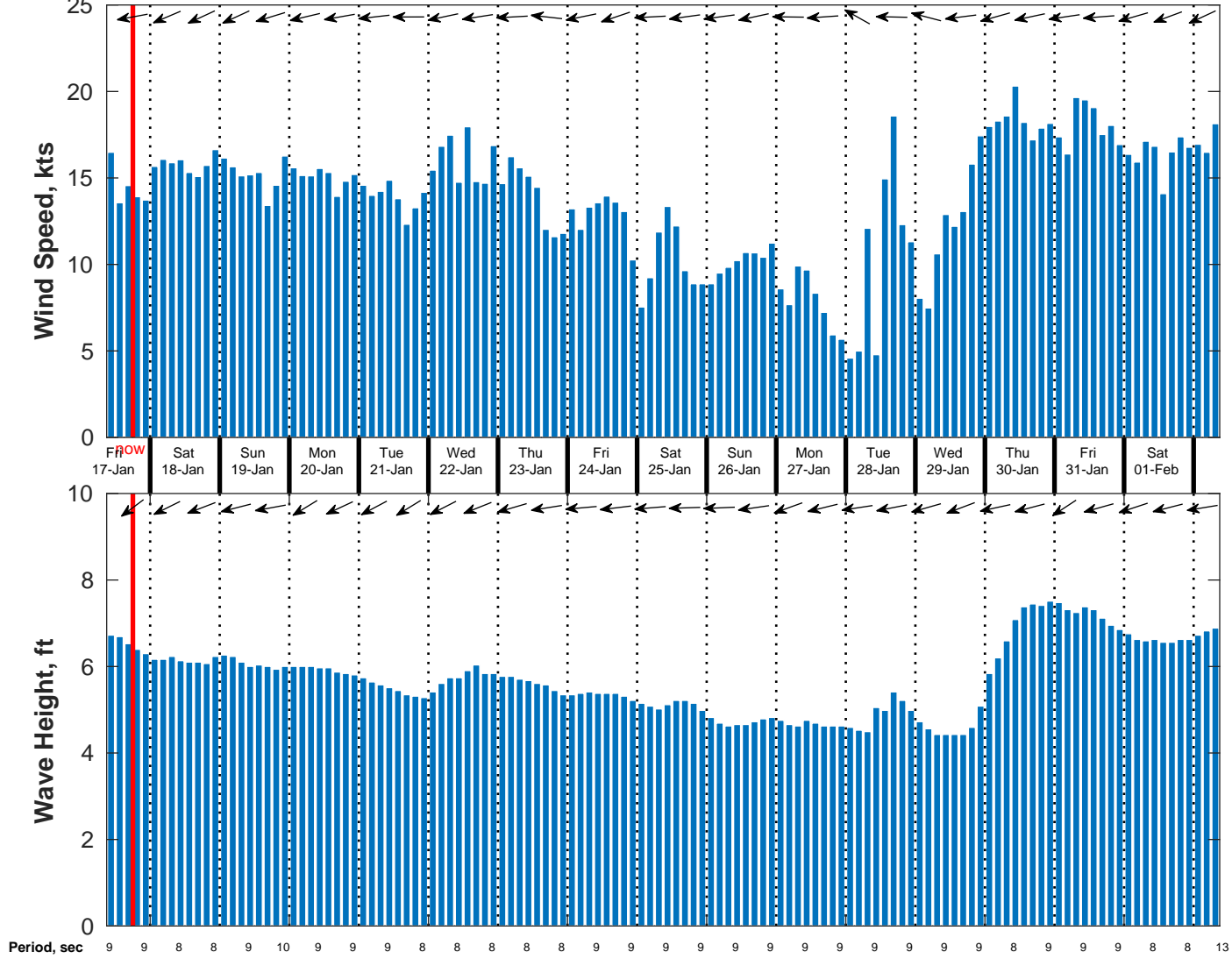
Wind & Wave Forecast for NDBC 52212 from 16-Jan-2025 09:00:00 to 01-Feb-2025 09:00:00
