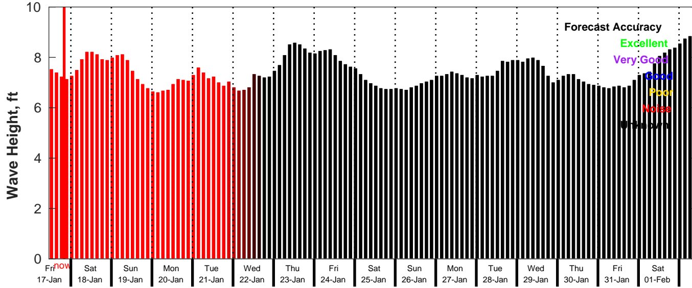
GFS Wave Forecast for NDBC 52213 from 16-Jan-2025 11:00:00 to 01-Feb-2025 11:00:00
