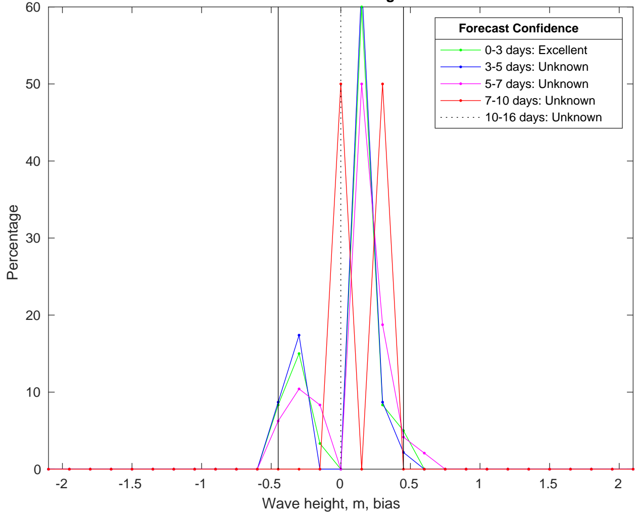
NDBC 62305 vs CMEMSWaves Bias Histogram: 16-Jan-2025
