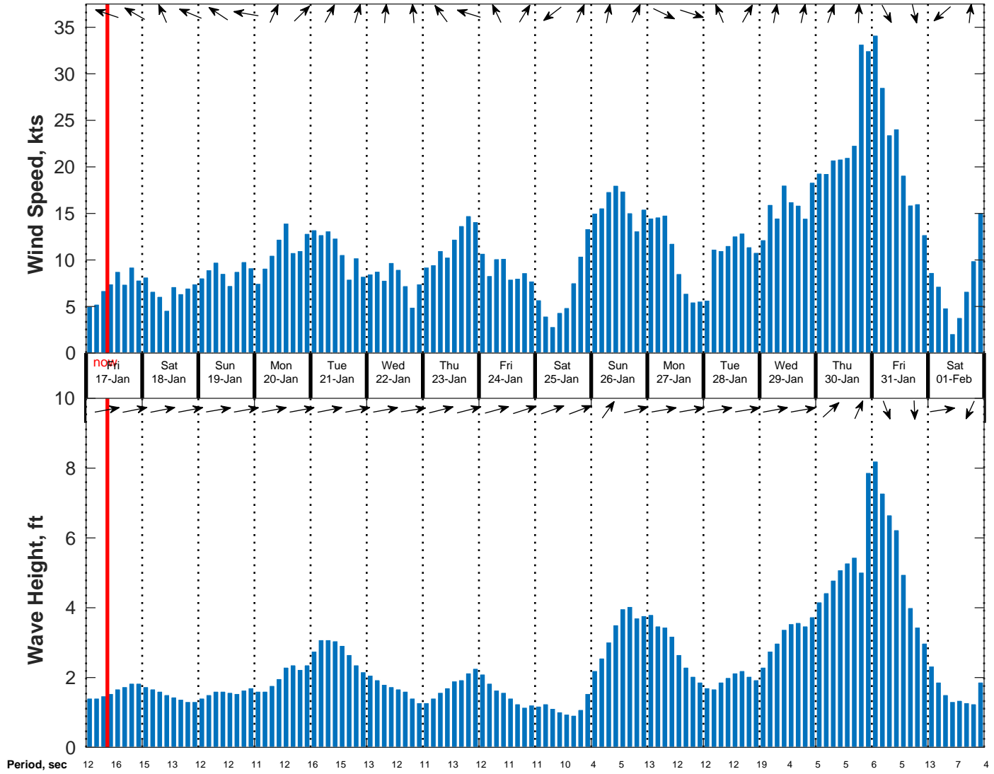
Wind & Wave Forecast for NDBC 62305 from 16-Jan-2025 00:00:00 to 01-Feb-2025 00:00:00
