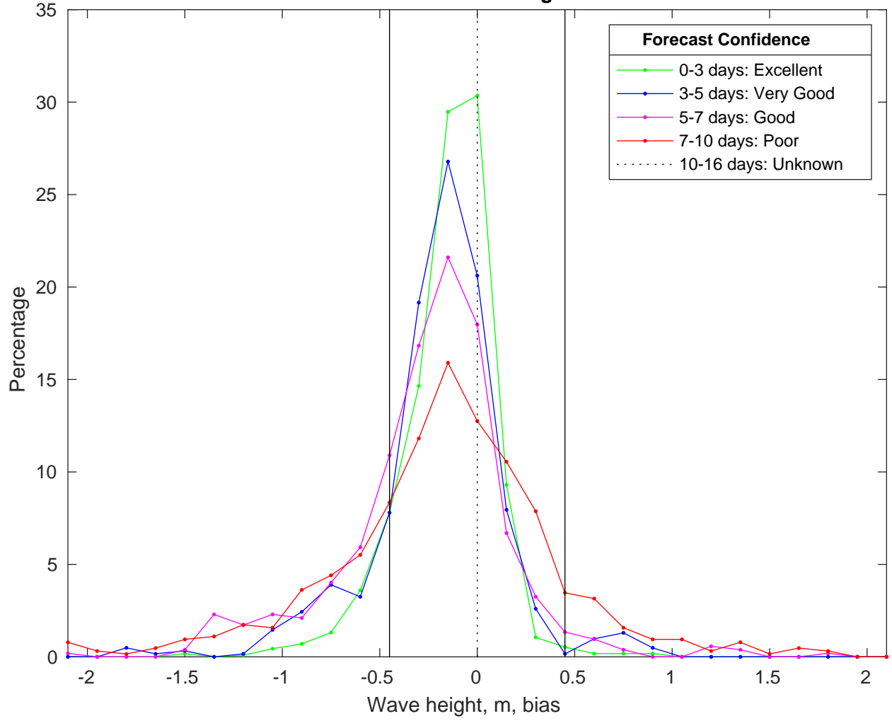
NDBC 41004 vs CMEMSWaves Bias Histogram: 17-Jan-2025
