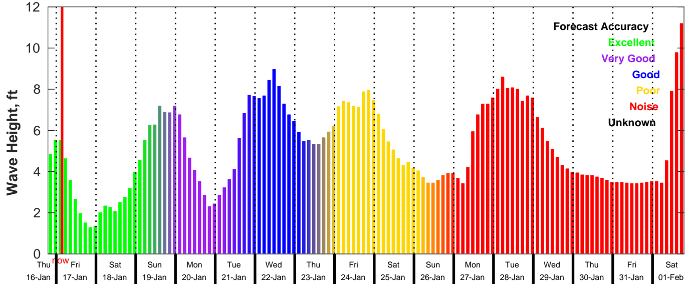
GFS Wave Forecast for NDBC 41004 from 16-Jan-2025 19:00:00 to 01-Feb-2025 19:00:00
