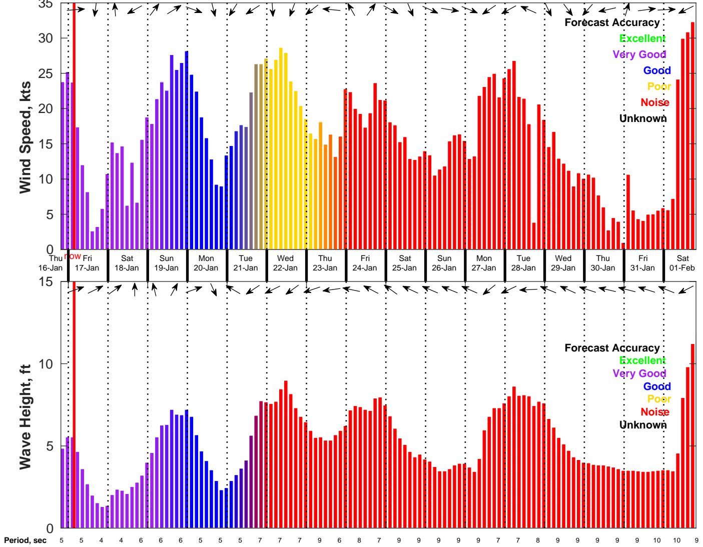
Wind & Wave Forecast for NDBC 41004 from 16-Jan-2025 19:00:00 to 01-Feb-2025 19:00:00
