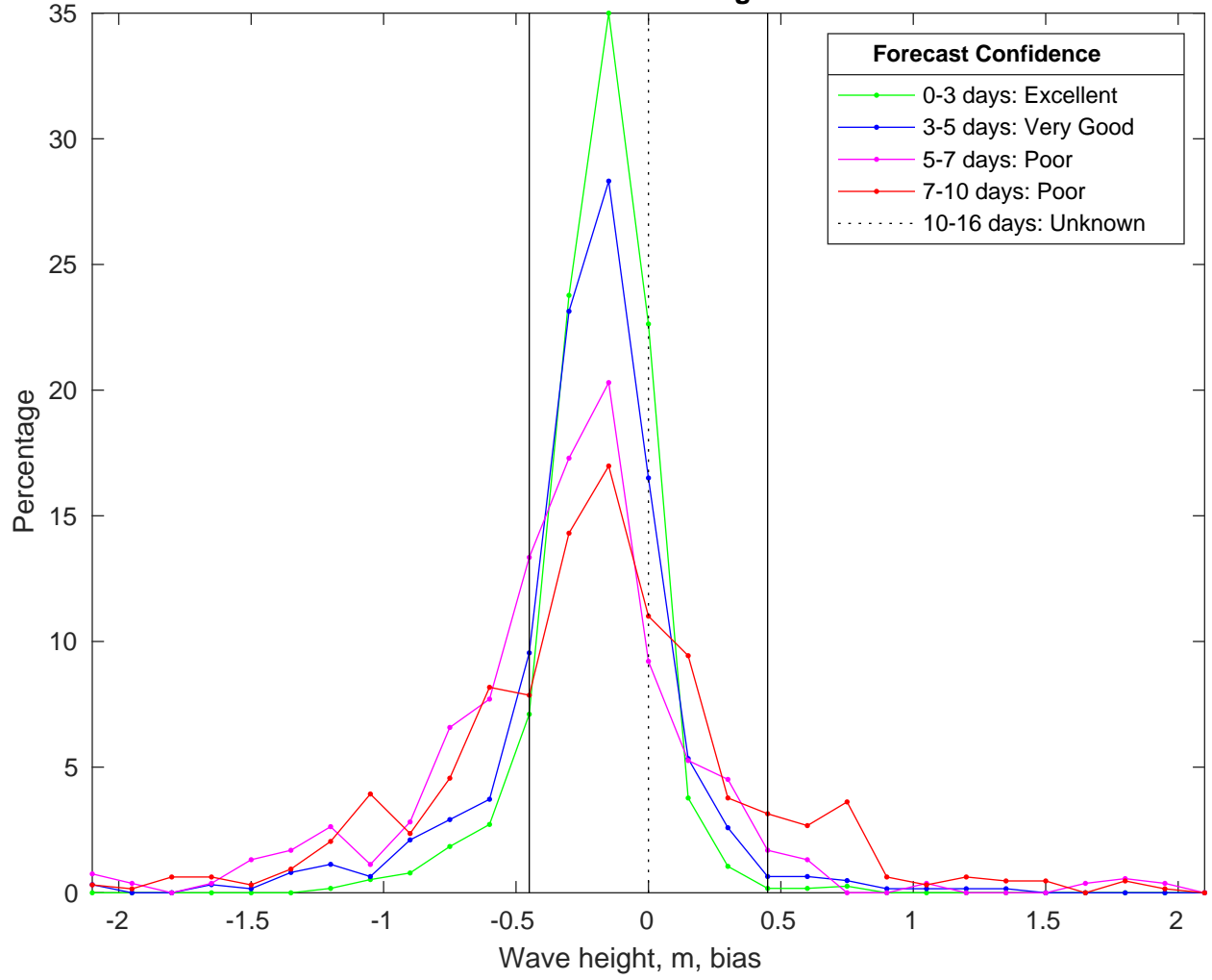
NDBC 41013 vs CMEMSWaves Bias Histogram: 17-Jan-2025
