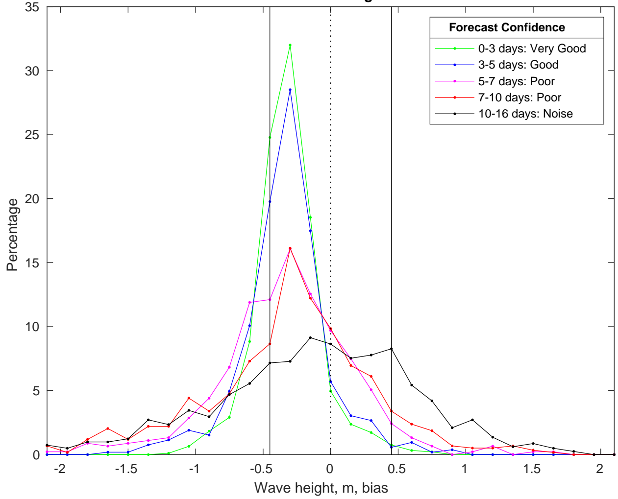
NDBC 41013 vs GFSWaves Bias Histogram: 17-Jan-2025
