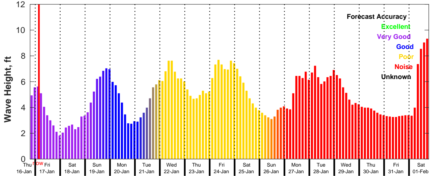
GFS Wave Forecast for NDBC 41013 from 16-Jan-2025 19:00:00 to 01-Feb-2025 19:00:00
