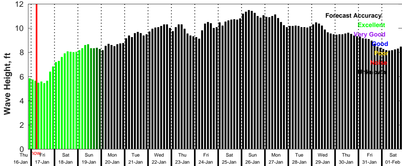
GFS Wave Forecast for NDBC 41040 from 16-Jan-2025 21:00:00 to 01-Feb-2025 21:00:00
