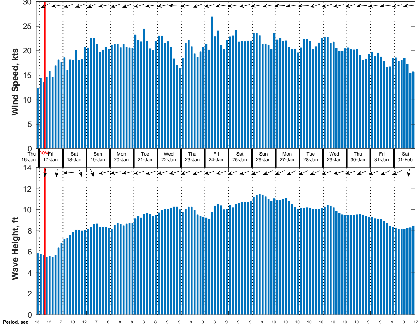
Wind & Wave Forecast for NDBC 41040 from 16-Jan-2025 21:00:00 to 01-Feb-2025 21:00:00
