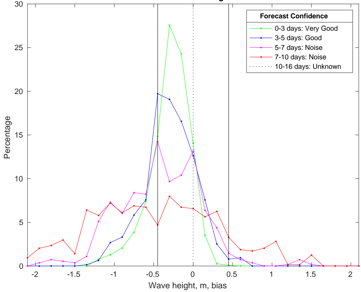
NDBC 42019 vs CMEMSWaves Bias Histogram: 17-Jan-2025
