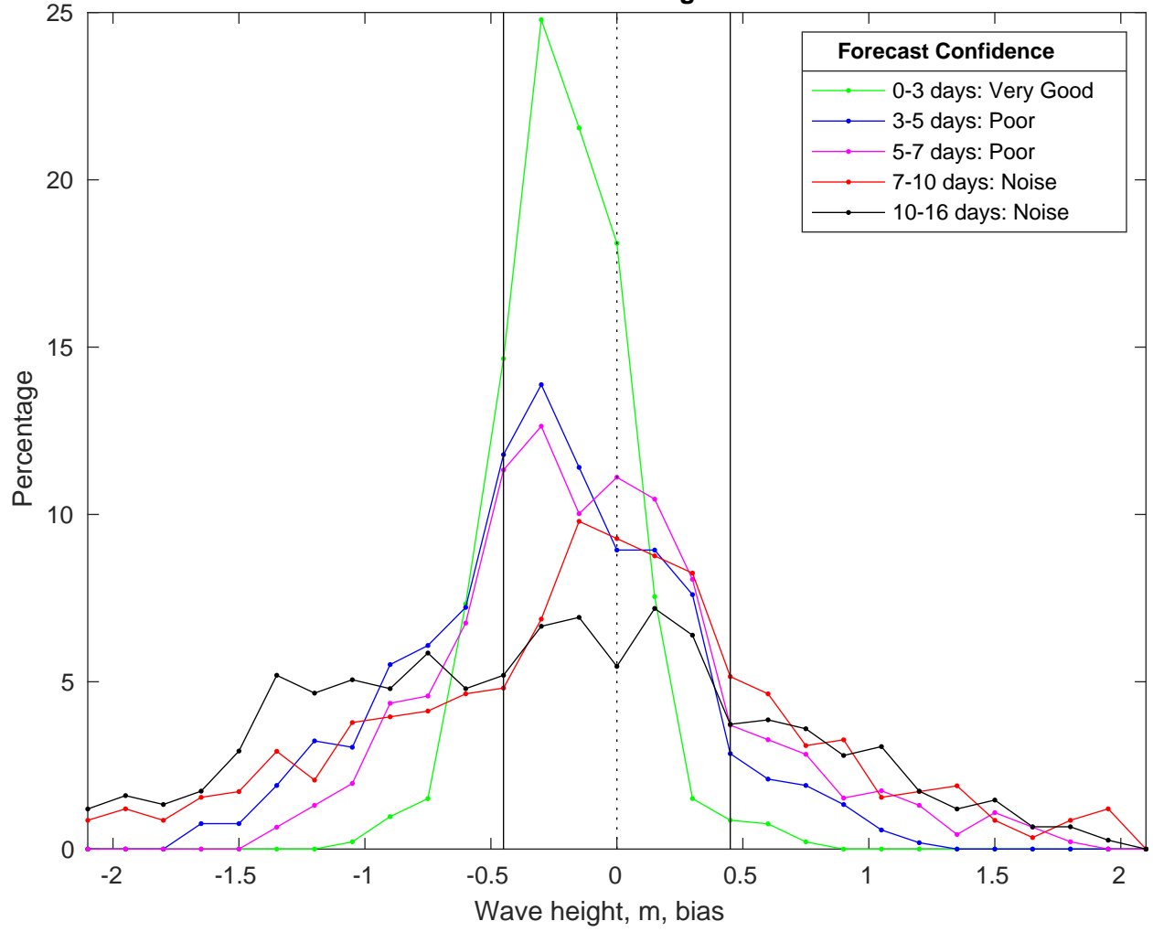
NDBC 42019 vs GFSWaves Bias Histogram: 17-Jan-2025
