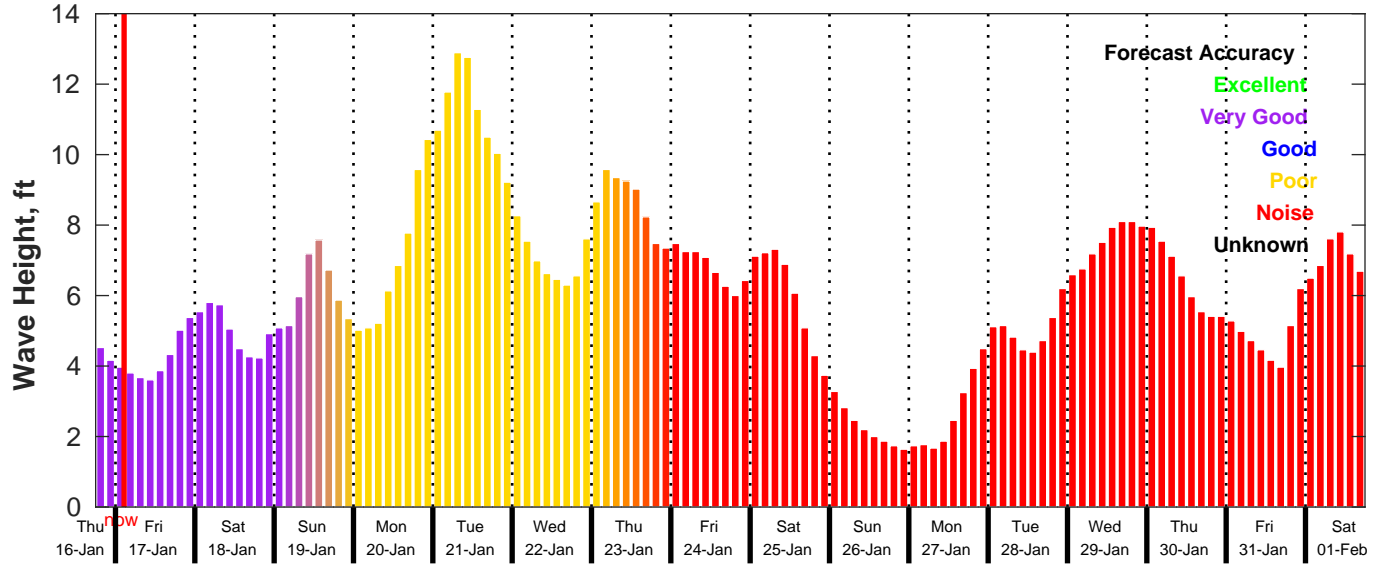
GFS Wave Forecast for NDBC 42019 from 16-Jan-2025 18:00:00 to 01-Feb-2025 18:00:00
