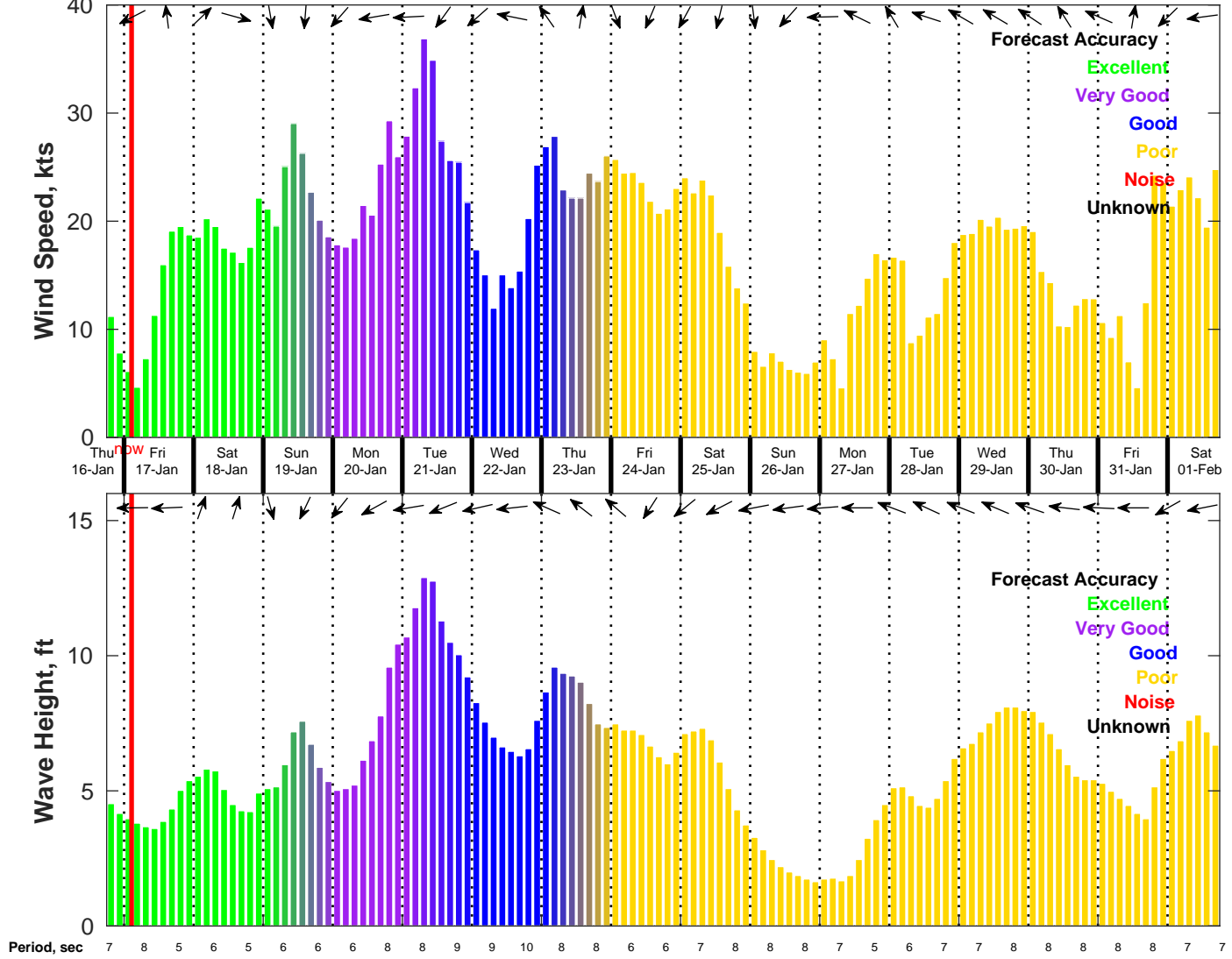
Wind & Wave Forecast for NDBC 42019 from 16-Jan-2025 18:00:00 to 01-Feb-2025 18:00:00
