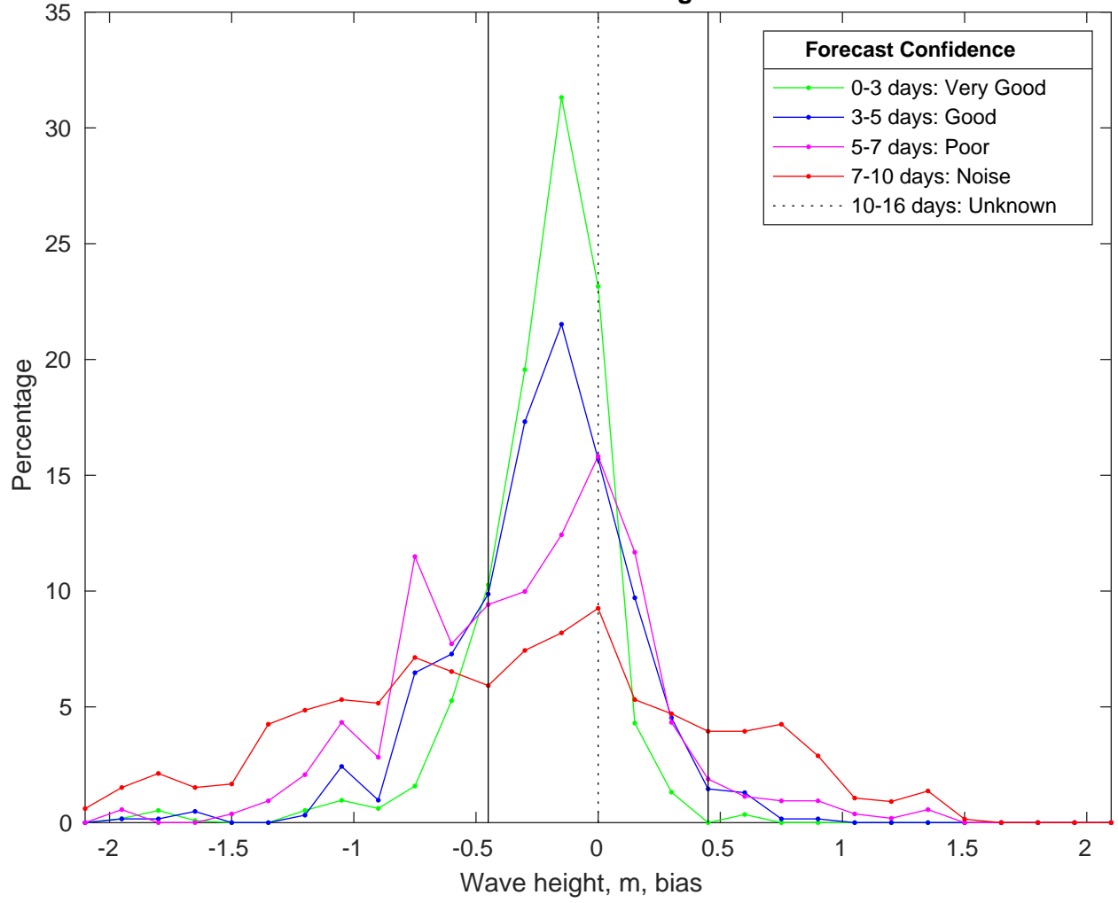
NDBC 42020 vs CMEMSWaves Bias Histogram: 17-Jan-2025
