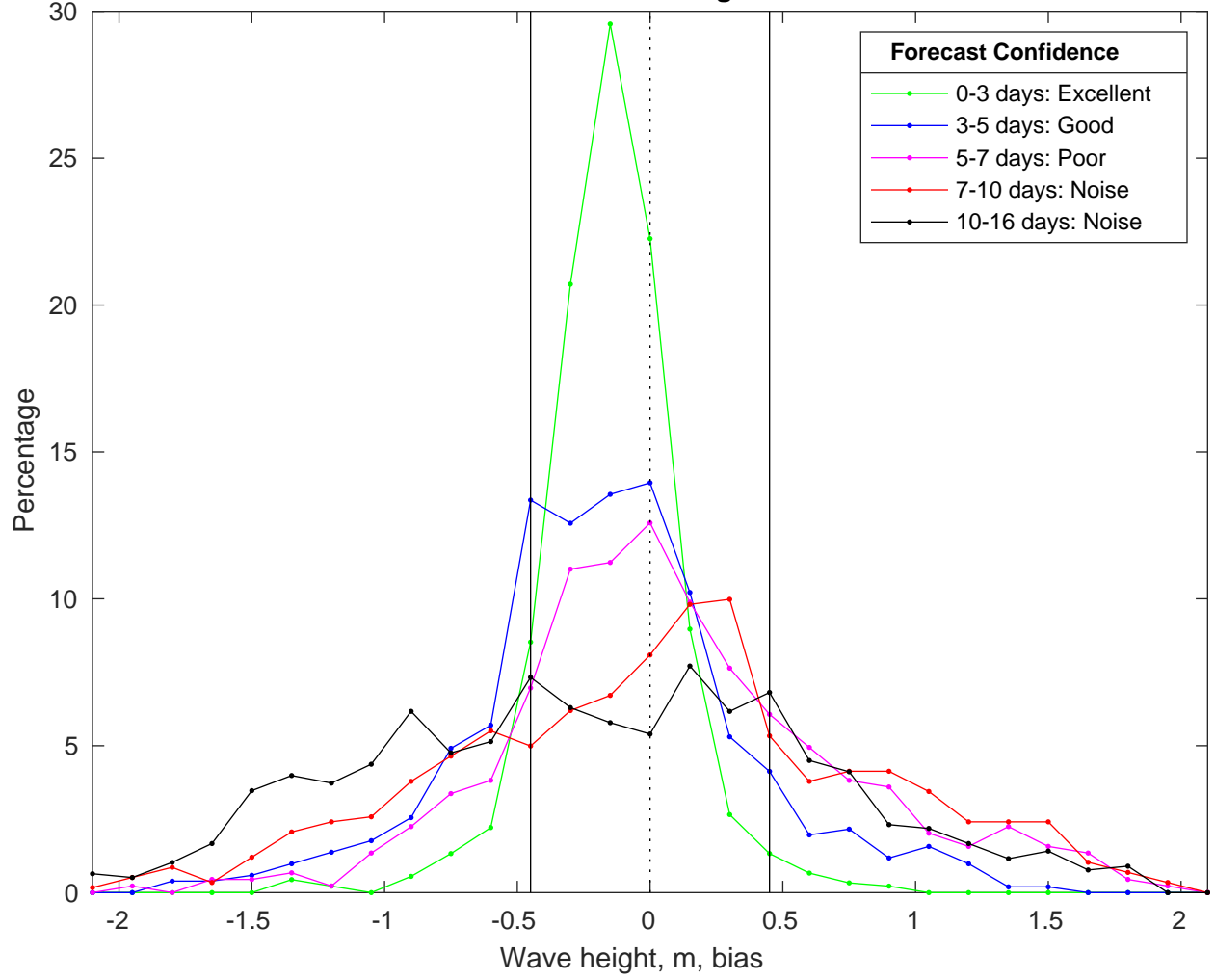
NDBC 42020 vs GFSWaves Bias Histogram: 17-Jan-2025
