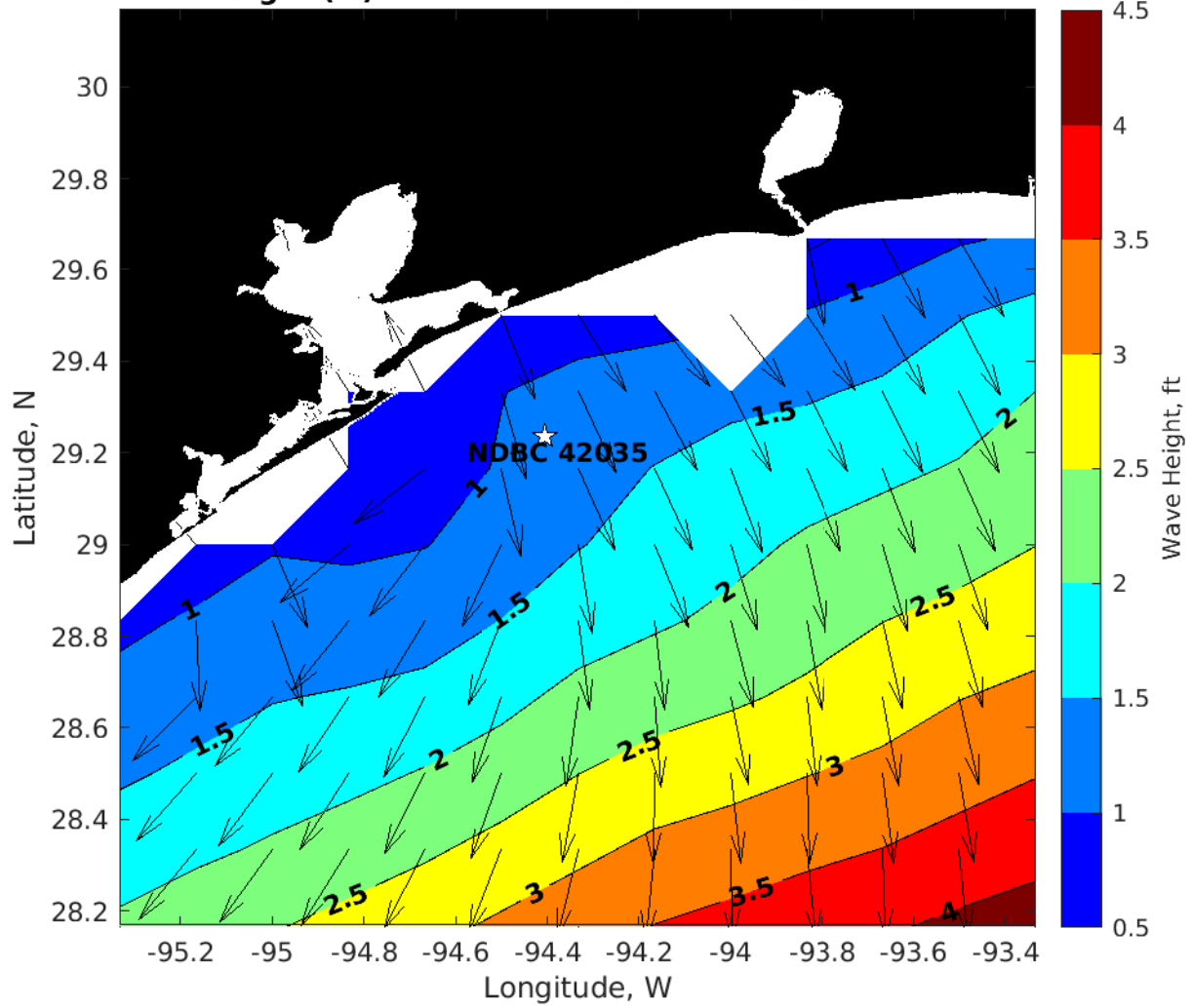
Wave Height (ft) for NDBC 42035 at 12-Dec-2024 00:00:00
