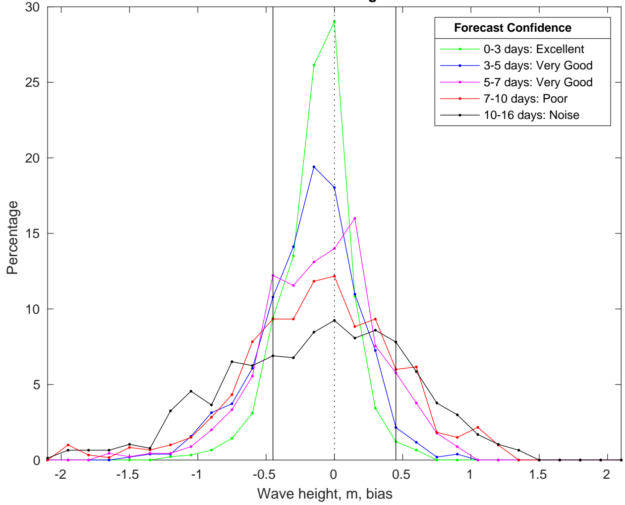
NDBC 42035 vs GFSWaves Bias Histogram: 17-Jan-2025
