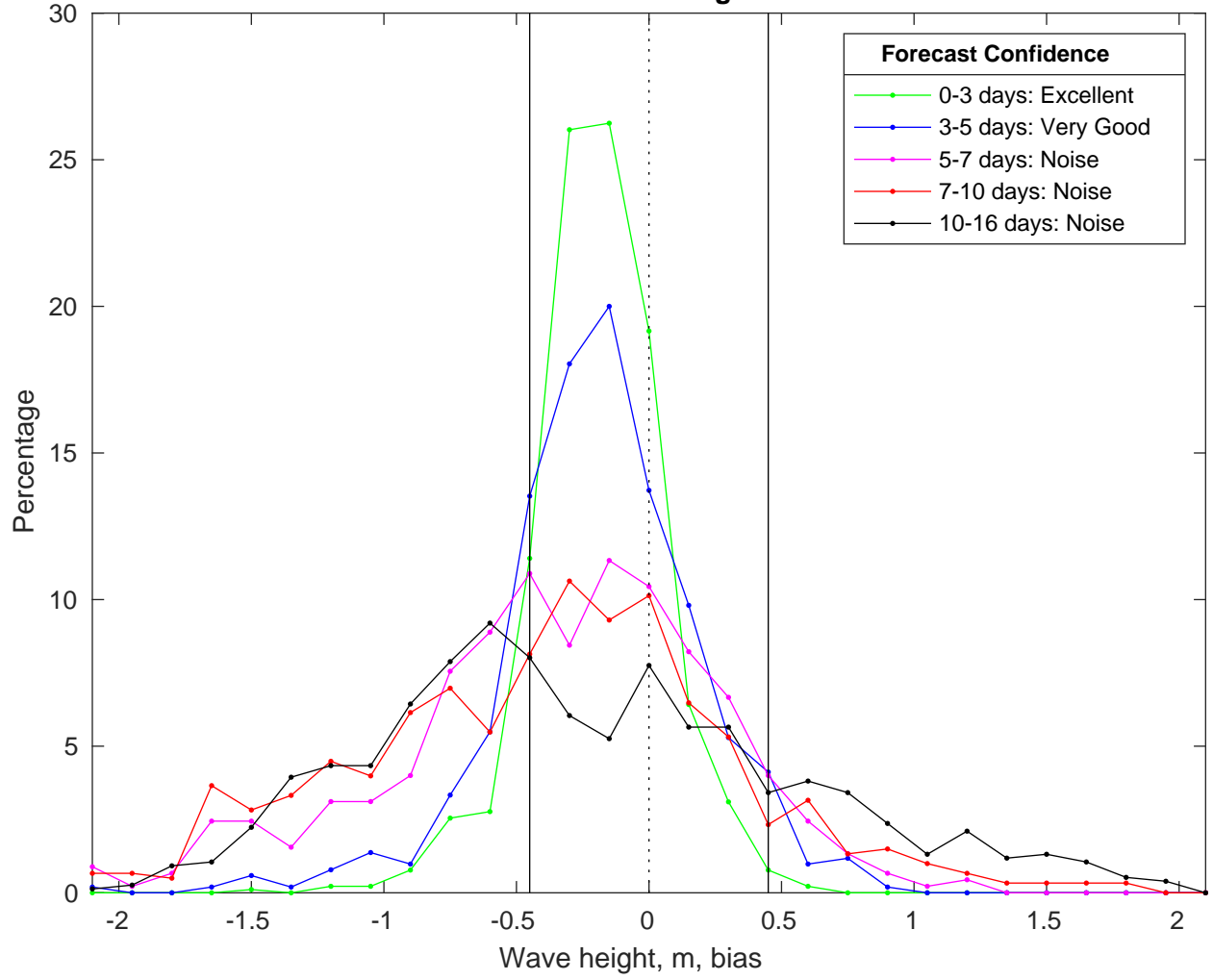
NDBC 42036 vs GFSWaves Bias Histogram: 17-Jan-2025
