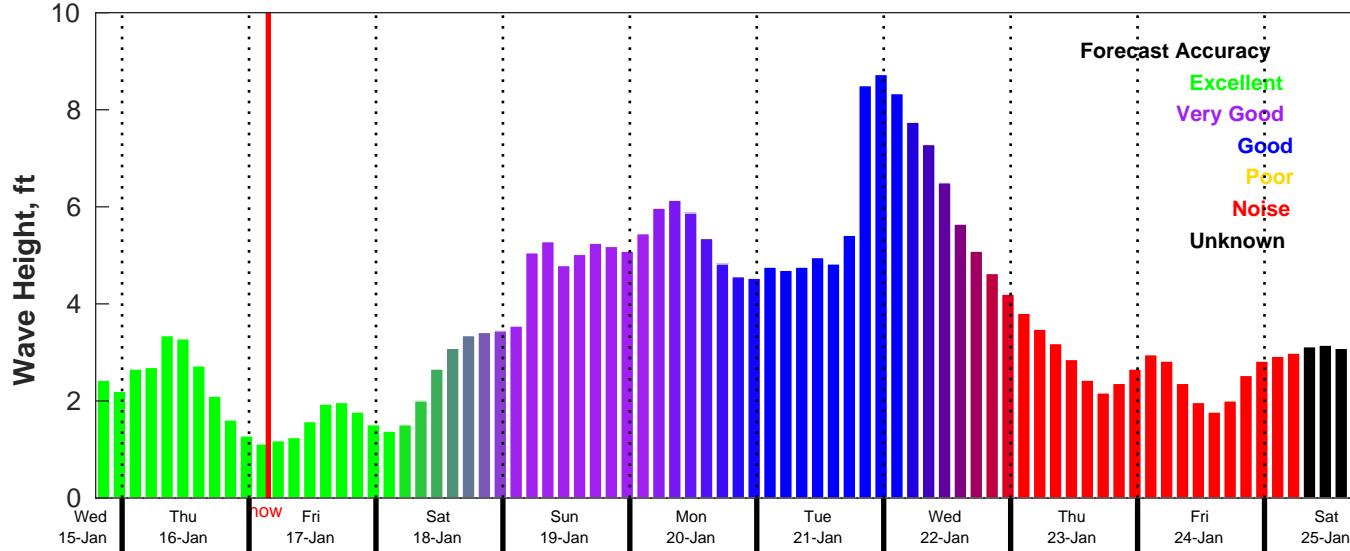
CMEMS Wave Forecast for NDBC 42036 from 15-Jan-2025 19:00:00 to 25-Jan-2025 19:00:00
