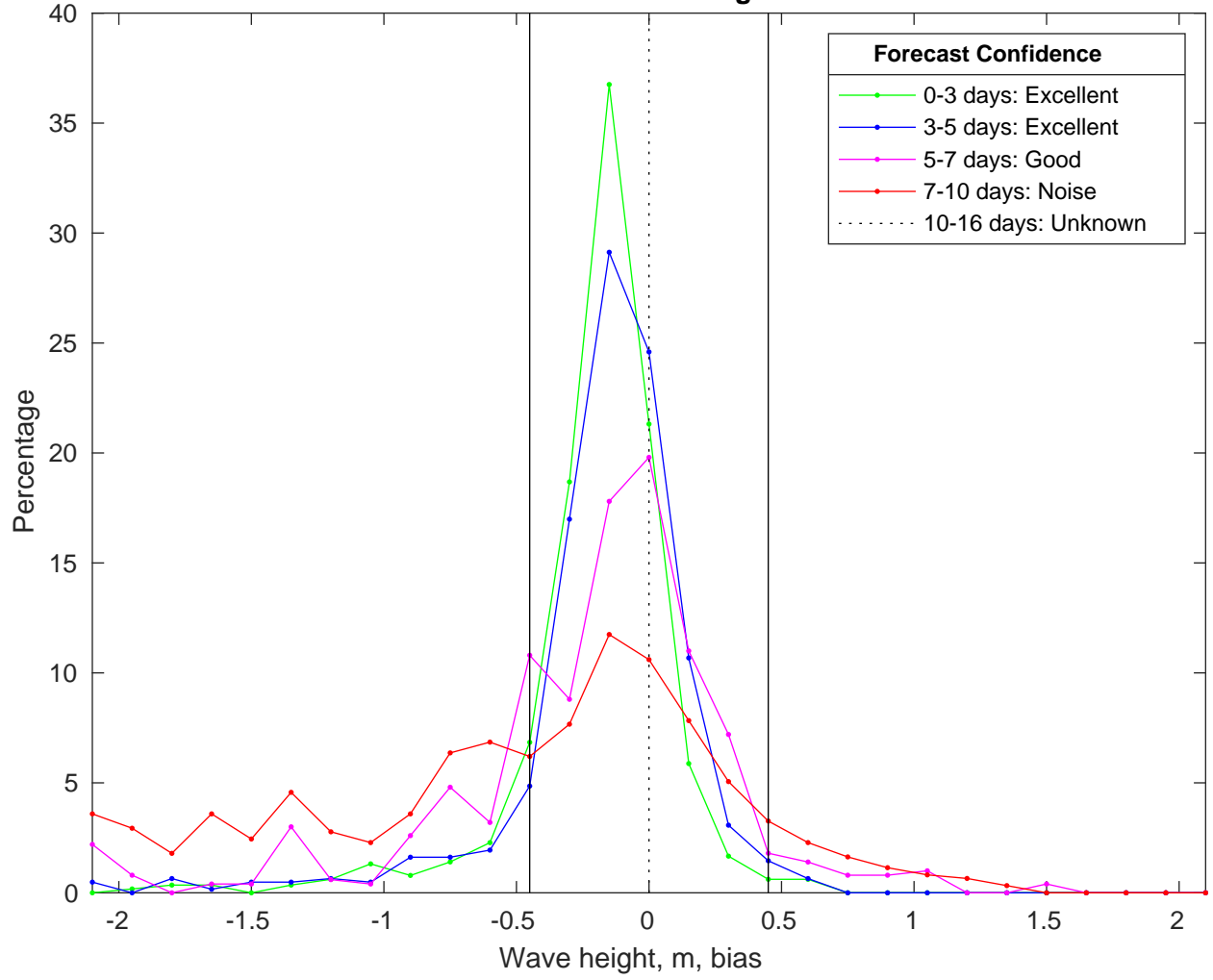
NDBC 42040 vs CMEMSWaves Bias Histogram: 17-Jan-2025
