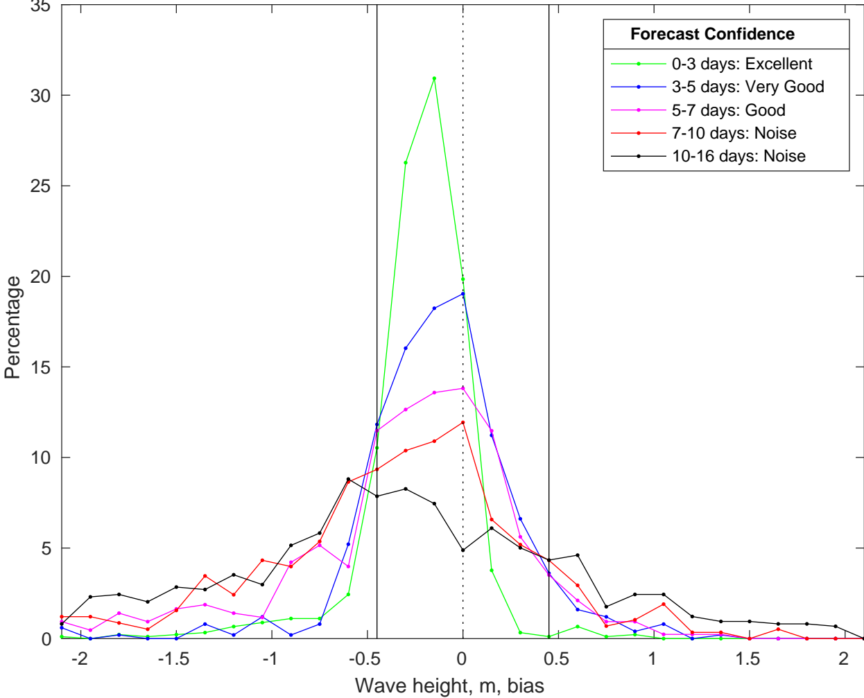
NDBC 42040 vs GFSWaves Bias Histogram: 17-Jan-2025
