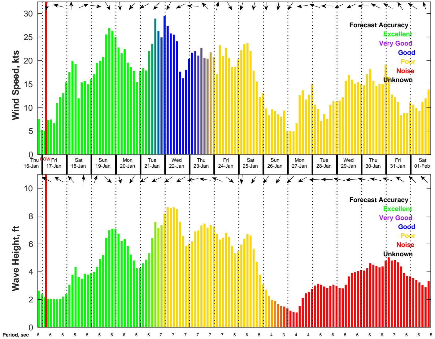
Wind & Wave Forecast for NDBC 42040 from 16-Jan-2025 19:00:00 to 01-Feb-2025 19:00:00
